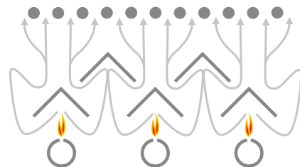
The slightly rising position of the sear plates allows naturally hotter air at the back to move to the front and balance out the difference in temperature.
