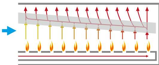
The upper sear plates circulate the hot air from the burners so that the area between burners gets hot enough as well.
